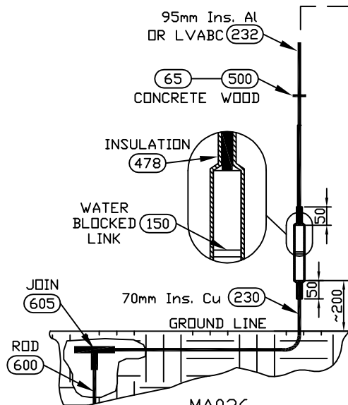
MA036 (OH TO UG EARTHING INSULATED BI-METAL JOINT) REFER ALSO TO SDI 100
