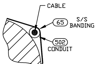
MA038 (CABLE SADDLE/SUPPORT + INS) FOR WOOD POLES USE SADDLES FOR CONCRETE POLES USE S/S BANDING
