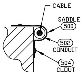
MA038 (CABLE SADDLE/SUPPORT + INS) FOR WOOD POLES USE SADDLES FOR CONCRETE POLES USE S/S BANDING
