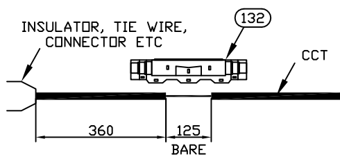
MA050 (CCT EARTH POINT)
