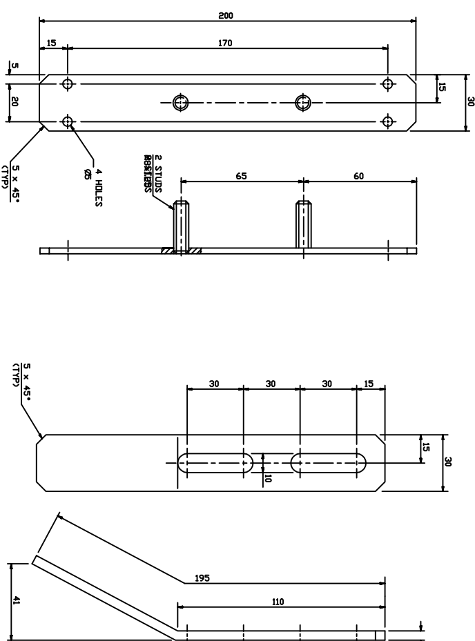
DOOR LOWER SECURITY PLATE DETAILS
