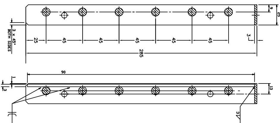
SECTION X-X
