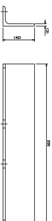
DOOR LATCH STRICKER PLATE RETAINING DETAIL ITEM 6 - DRG. No 264890
