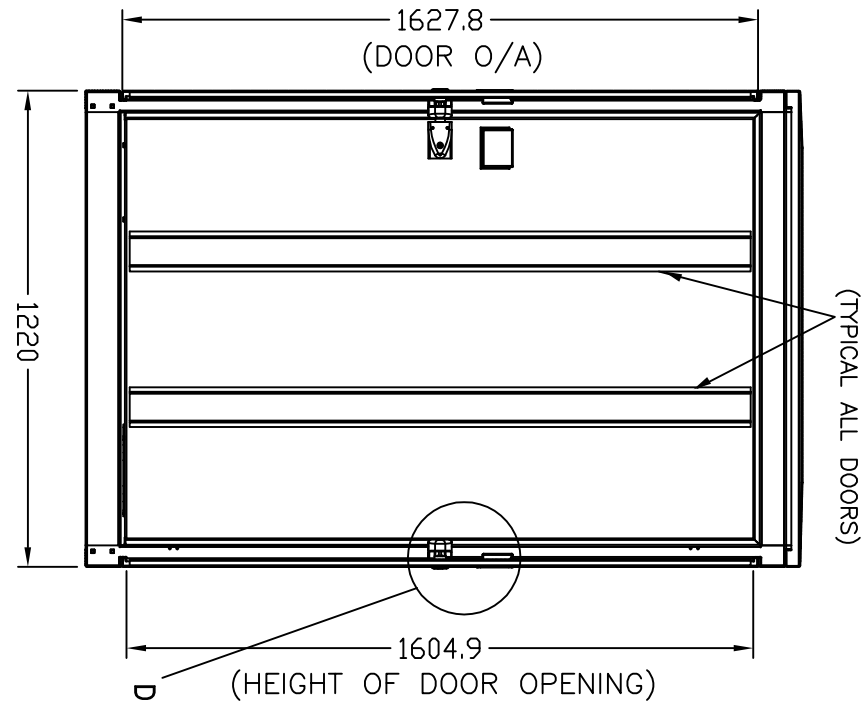
SECTION C-C
