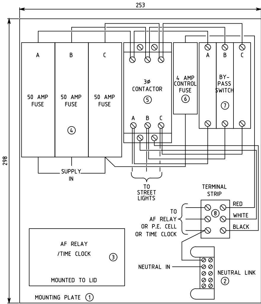
THREE PHASE STREETLIGHT CONTROL POINT - EQUIPMENT LAYOUT
