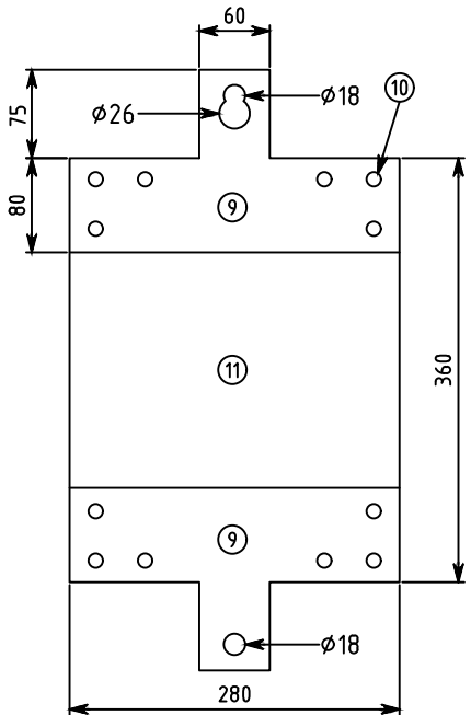
CONTROL POINT ENCLOSURE - REAR VIEW
