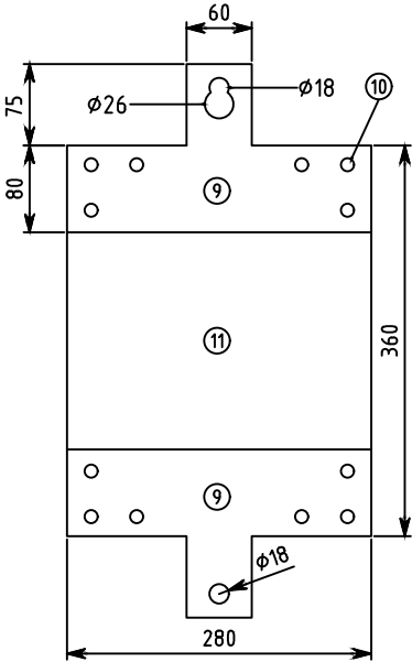
CONTROL POINT ENCLOSURE - REAR VIEW
