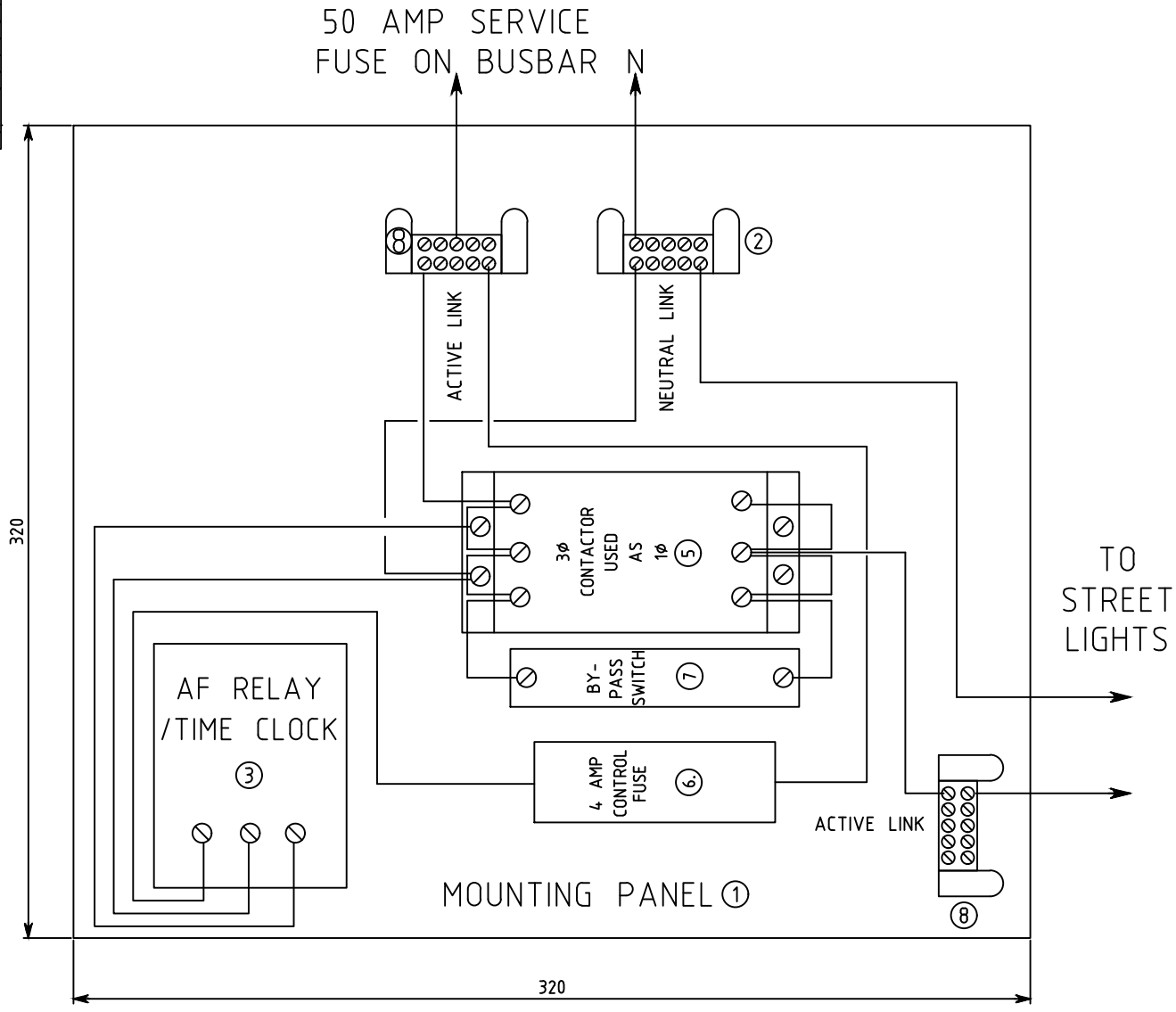
SINGLE PHASE STREETLIGHTS CONTROL POINT - EQUIPMENT LAYOUT
