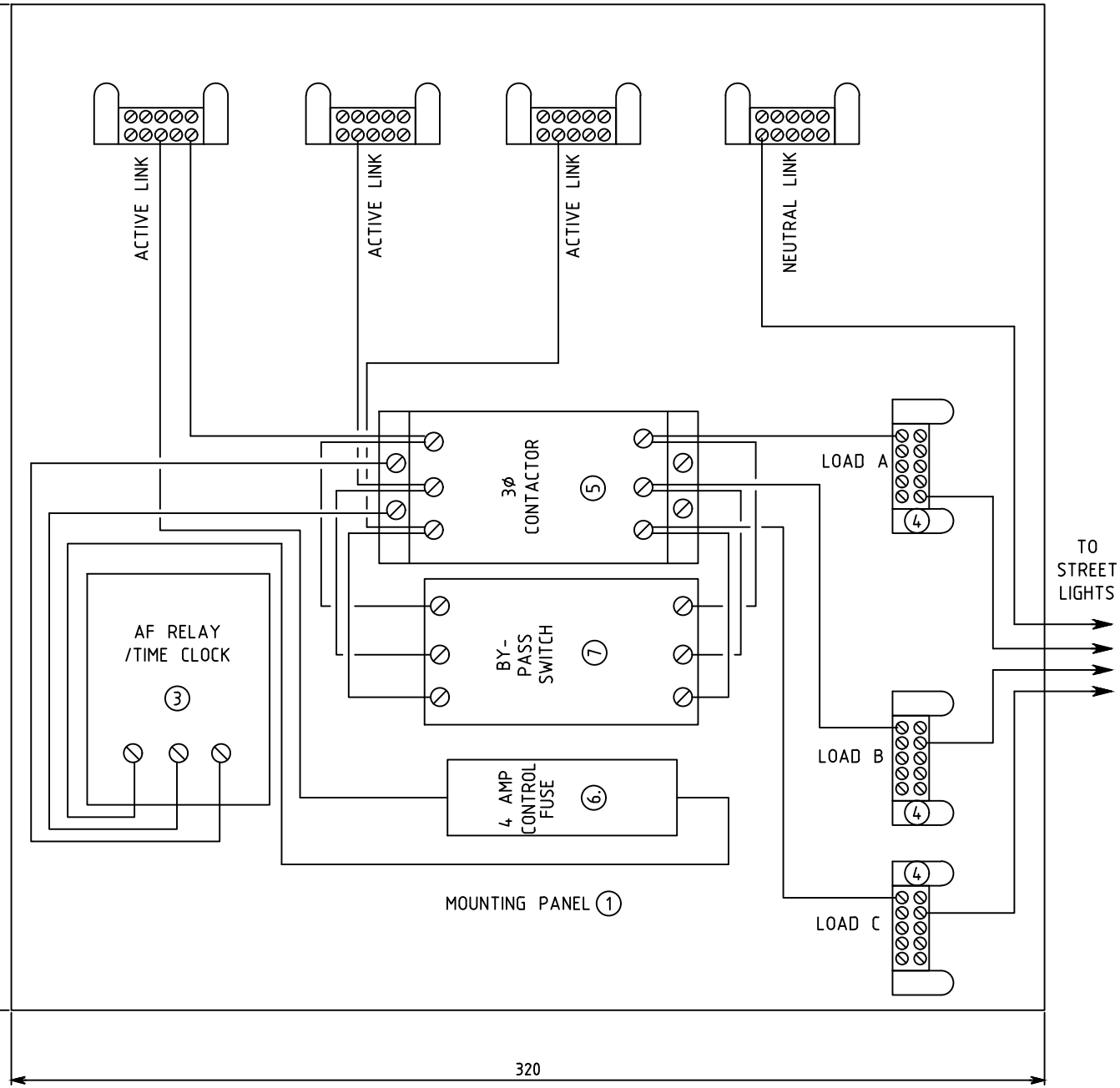
THREE PHASE STREETLIGHTS CONTROL POINT - EQUIPMENT LAYOUT
