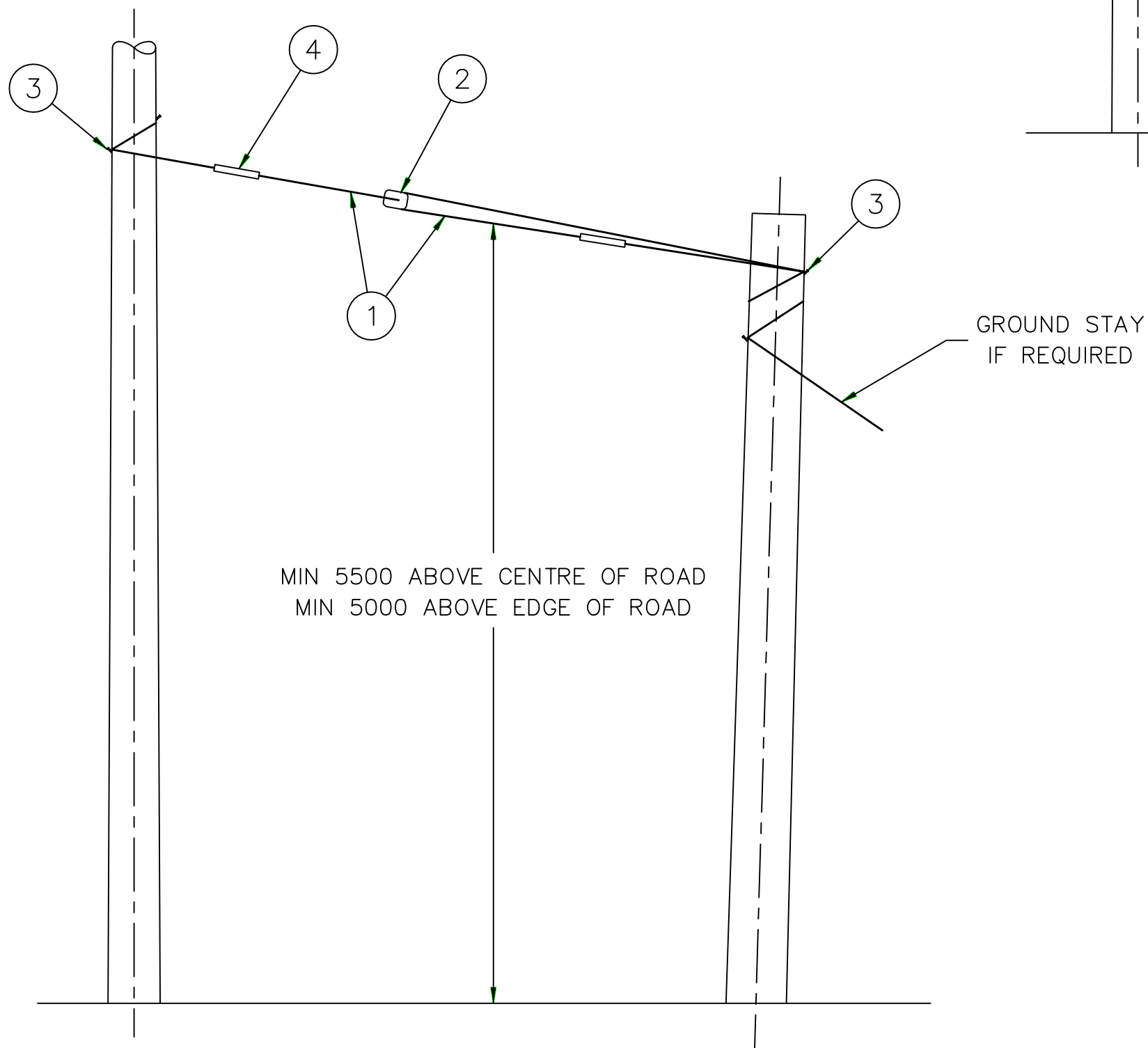
AERIAL STAY TYPES A2 & A3 (DOUBLE WIRE)
