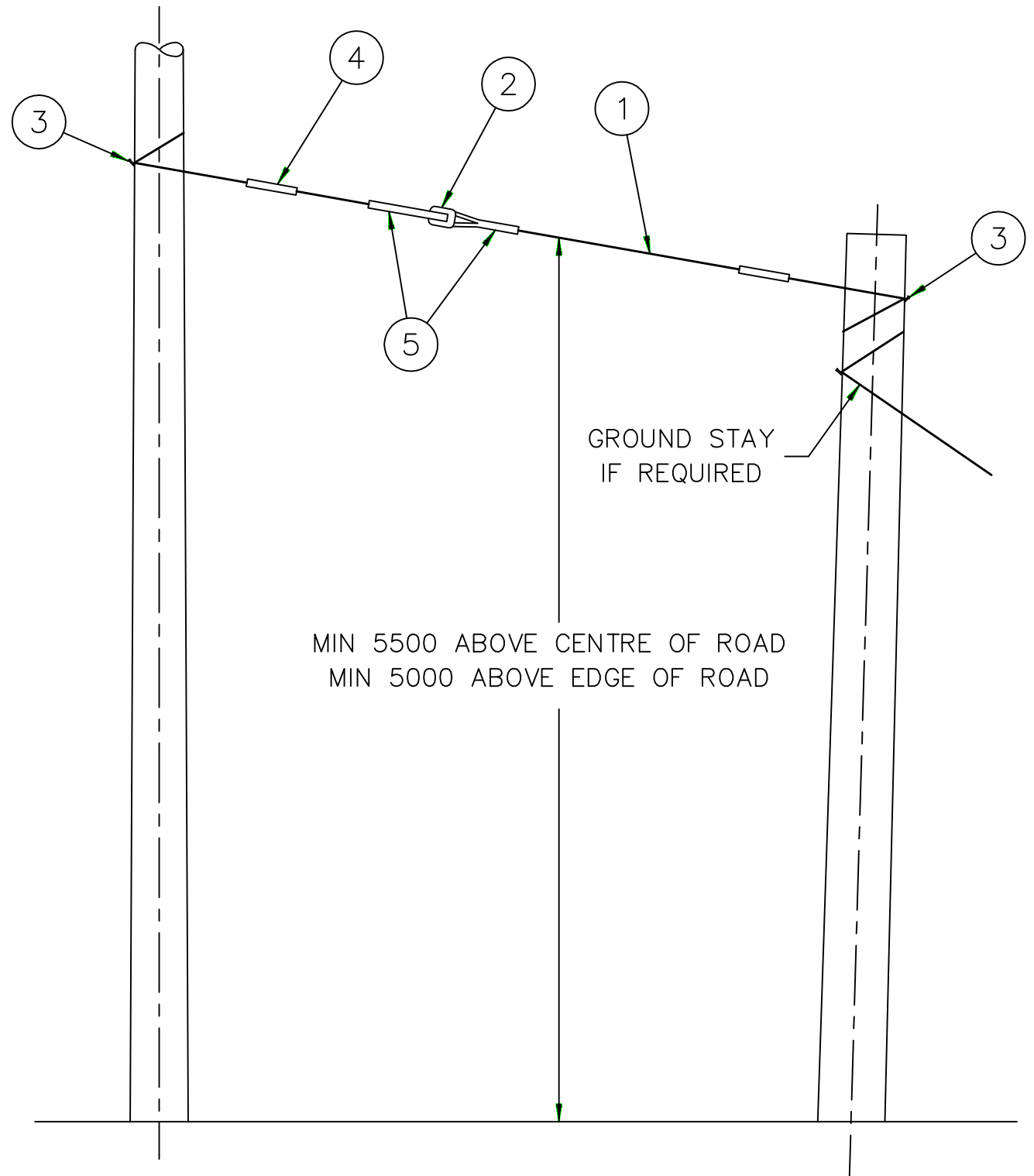
AERIAL STAY TYPE A1 (SINGLE WIRE)
