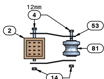
IA002-102 (INS. SHACKLE LV - STRAP)
