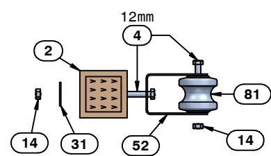
IA004-102 (INS. SHACLE LV - 'D')
