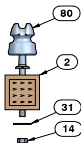
IA001-101 (INS. LONG PIN LV)
