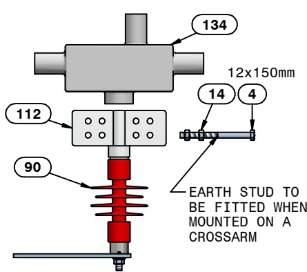
IA015 (INS. WITH PALM + COVER) EARTH STUD TO BE FITTED WHEN MOUNTED ON A CROSSARM, BUT COVER THEN NOT REQ.
