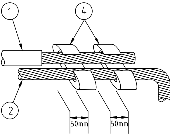
EARTHING CLAMPS - DETAIL B
