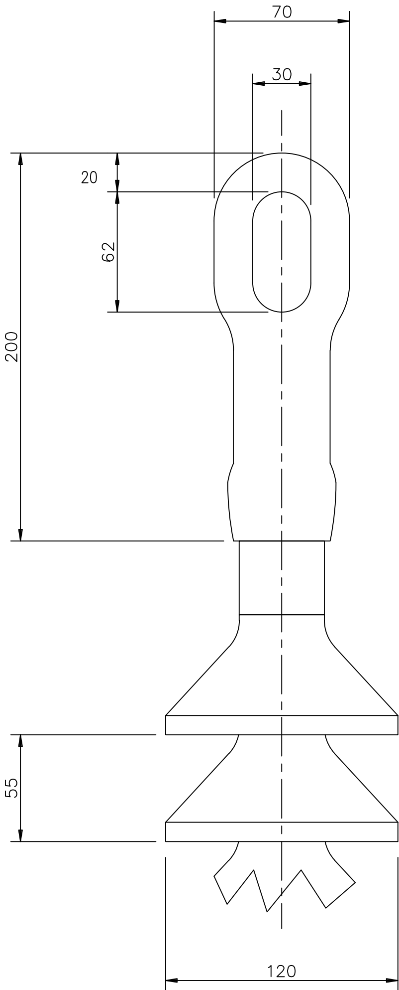
'EYE' TYPE END FITTING DETAIL SCALE 1:2
