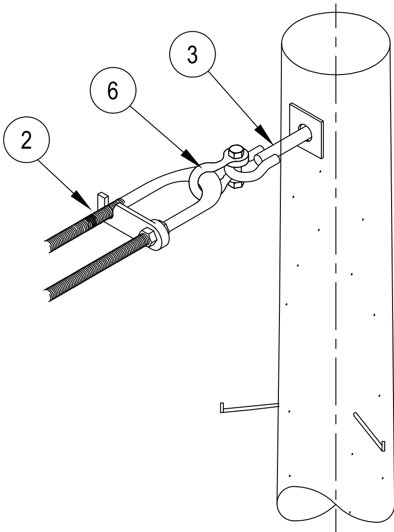
ALTERNATIVE ARRANGEMENT FOR EYEBOLT.
