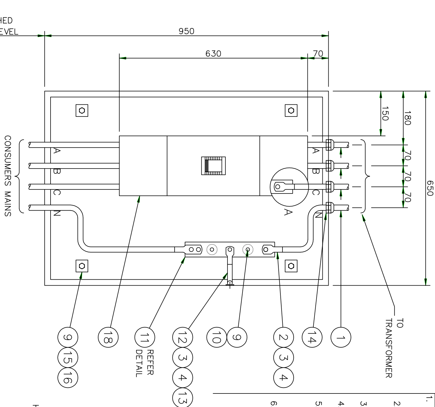
INTERNAL EQUIPMENT ARRANGEMENT
