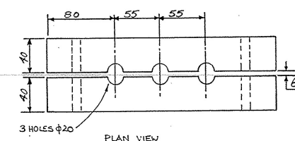
PLAN VIEW
