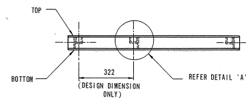
DETAIL ITEM 1 SUPPORT PLINTH ASSEMBLY SCALE 1:10
