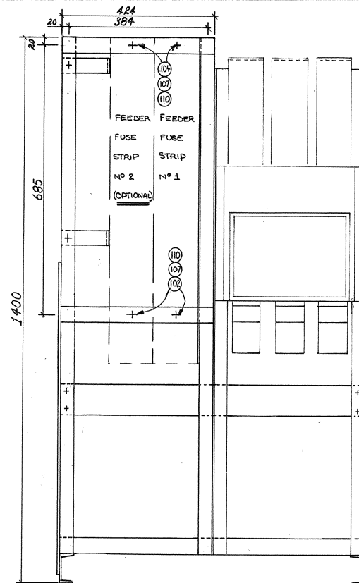
TOP VIEW (C.B. & M.O.I. OMITTED)
