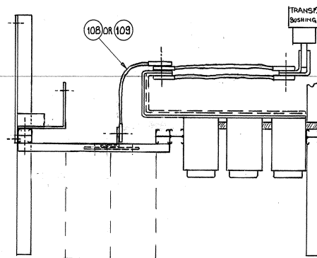
TOP VIEW (C.B. & M.O.I. OMITTED)
